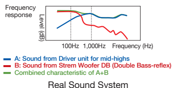
Stream Woofer DB (Double Bass-reflex)
